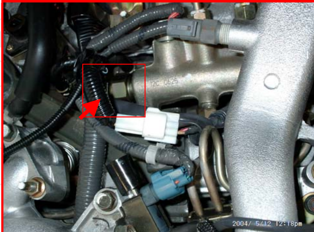
Close up plug (6 Pin) at the common rail strip
